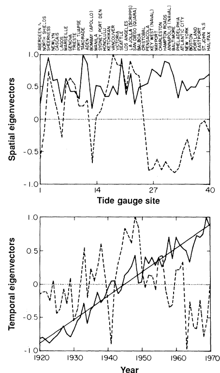
Fig. 8. Same as for Fig. 7 but for the reduced data from the 40 tide gauge stations with records of 50 years' duration that remain once the Baltic data are eliminated. Two additional records (Wajima, Japan, and Astoria, Oregon) have also been eliminated.
